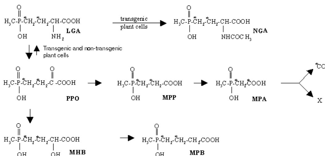
Figure 1. Degradation scheme proposed for the metabolism of L-glufosinate in cell cultures of sensitive and transgenic, glufosinate-resistant oilseed rape and corn (*C = ^{14}\text{C} -labeled, X = unknown metabolite).
